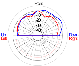
Polar Response - 2D 2KHz
