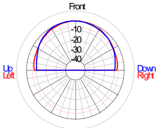
Polar Response - 2D 500Hz
