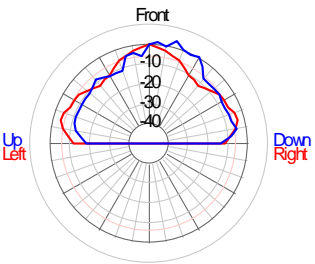
Polar Response - 2D 16KHz
