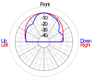
Polar Response - 2D 500Hz
