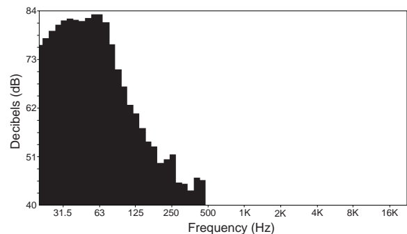
Figure 1: On-axis frequency response W/ 80Hz LPF.
